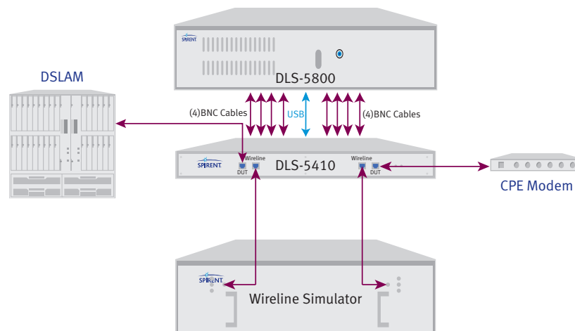
Physical Layer Test Setup including Wireline Simulation, Noise Generation, Traffic Generation and Analysis
