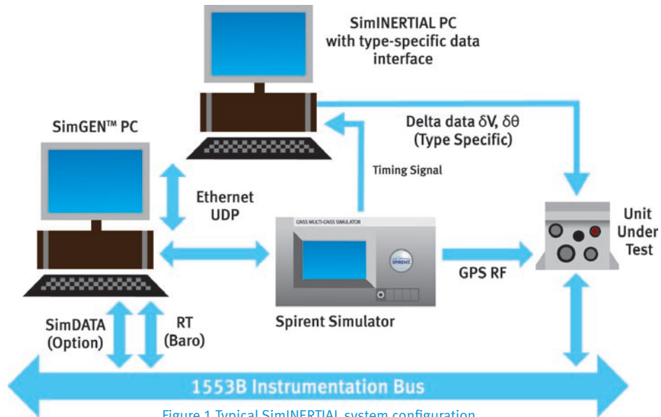
Figure 1 Typical SimINERTIAL system configuration
