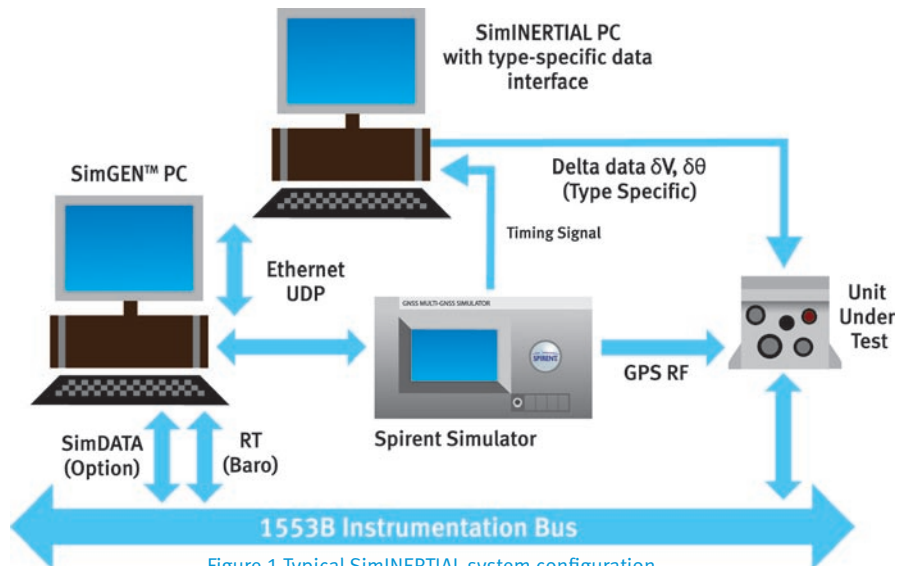
Figure 1 Typical SimINERTIAL system configuration
